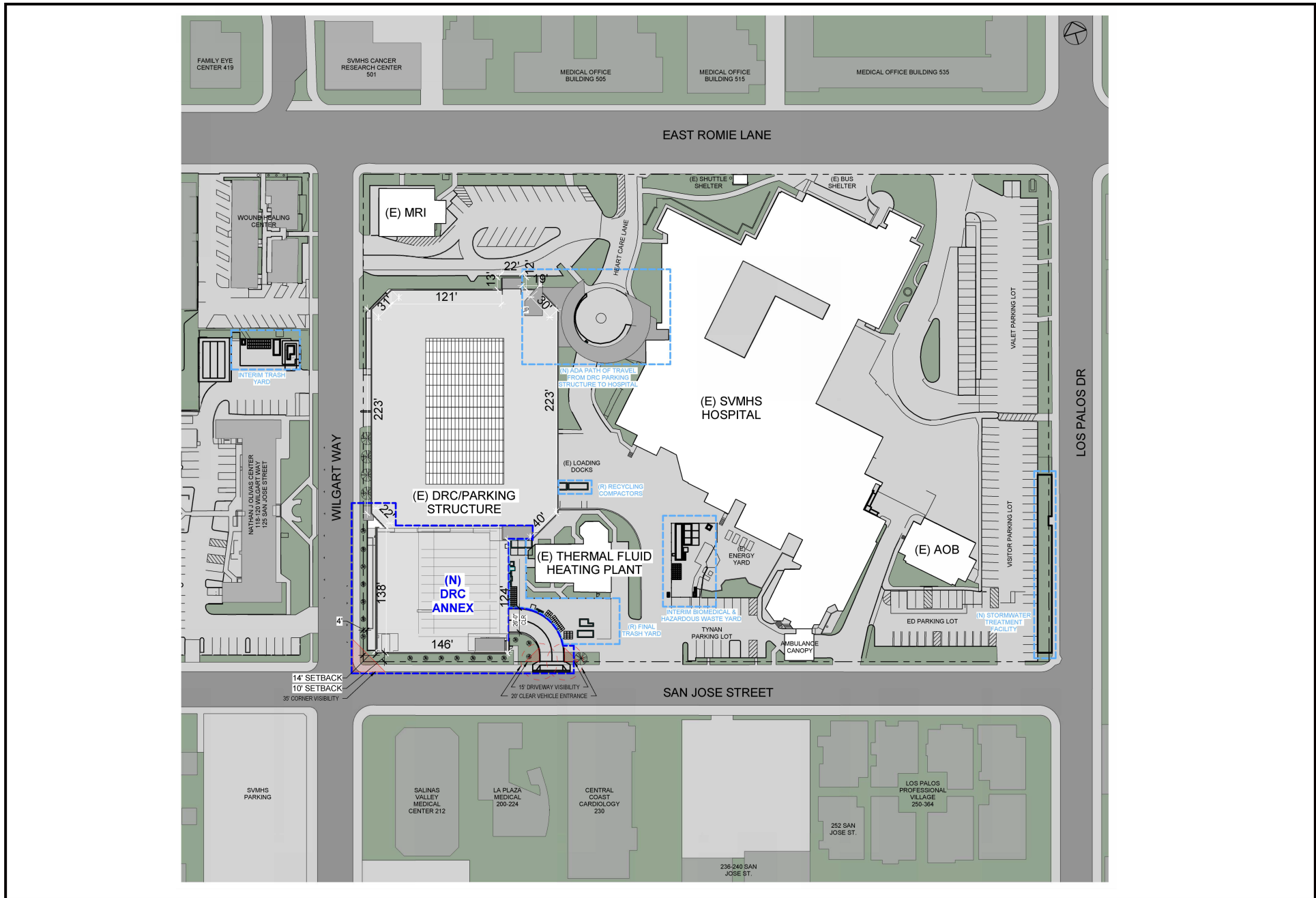
Figure 2: Proposed Site Plan Salinas Valley Memorial Healthcare System
